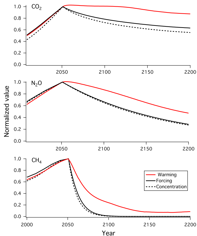
Fig. 2. Relative changes in CO 2 (Top), N 2 O (Middle) and CH 4 (Bottom) concentrations, radiative forcings, and surface warmings, normalized to one at their peak values, for the A1B scenario to 2050, followed by an abrupt cessation of emissions (as in Fig. 1).
